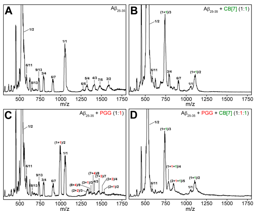
Figure 1. ESI-Q mass spectra of (A) pure A\beta_{25-35} , (B) A\beta_{25-35} incubated with CB[7] at 1:1, (C) A\beta_{25-35} incubated with PGG at 1:1, and (D) A\beta_{25-35} incubated with PGG and CB[7] at 1:1:1 molar ratio. The A\beta_{25-35} concentration was 100 \mu M in acidified water (0.1% (v/v) of formic acid) in all cases. The peaks of the A\beta_{25-35} homo-oligomers are annotated as ratios of the oligomer size n and the charge z , whereas the hetero-oligomer peaks of A\beta_{25-35} with ligands are annotated by (n+p)/z , (n+k)/z and (n+p+k)/z , where p and k are the numbers of PGG and CB[7] molecules, respectively.
