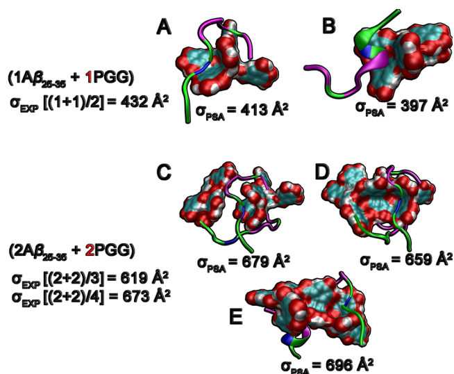
Figure 7. Representative structures of A\beta_{25-35} /PGG complexes obtained from simulations. (A, B) Heterodimers of one A\beta_{25-35} and one PGG. A\beta_{25-35} monomers adopt a wide range of structures from random coil to partial helix. (C–E) Heterotetramers of two A\beta_{25-35} and two PGG molecules. The PGG molecules are represented in filled surface with oxygens in red, carbon in cyan and hydrogen in white. The A\beta_{25-35} peptides are shown in cartoon representation where nonpolar residues are shown in pink, charged residues in blue, and polar residues in green.
