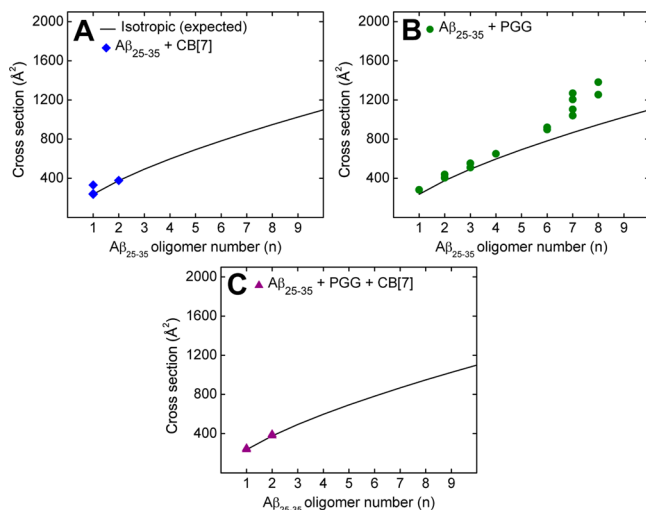
Figure 4. Oligomer growth curve data of hetero-oligomers of (A) A\beta_{25-35} incubated with CB[7] at 1:1, (B) A\beta_{25-35} incubated with PGG at 1:1, and (C) A\beta_{25-35} incubated with PGG and CB[7] at 1:1:1 molar ratio. The cross sections of A\beta_{25-35} oligomers reported here were extracted from the hetero-oligomer cross sections (see Supporting Information Tables S2–S4).
