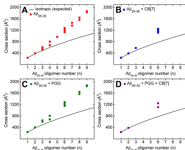
Figure 2. Oligomer growth curve data of the A\beta_{25-35} homo-oligomers of (A) pure A\beta_{25-35} , (B) A\beta_{25-35} incubated with CB[7] at 1:1, (C) A\beta_{25-35} incubated with PGG at 1:1, and (D) A\beta_{25-35} incubated with PGG and CB[7] at 1:1:1 molar ratio.
