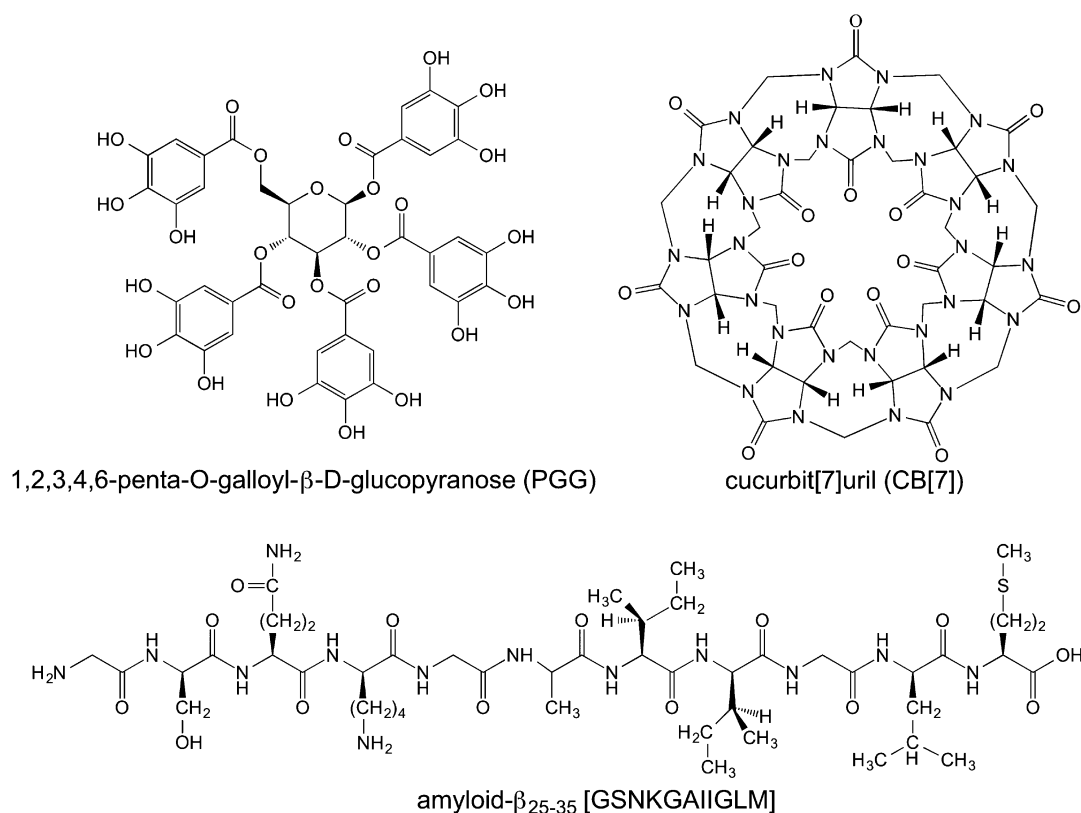
Scheme 1. Structural Formulas of 1,2,3,4,6-Penta-O-galloyl- \beta -D-glucopyranose (PGG), Cucurbit[7]uril (CB[7]), and A\beta_{25-35}
