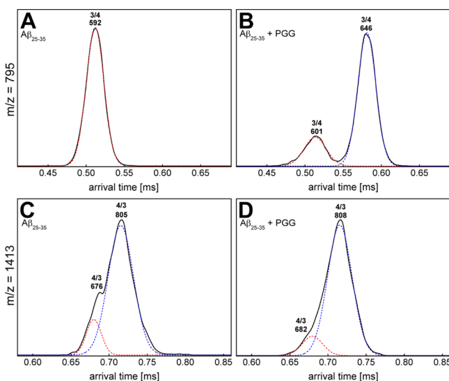
Figure 6. Representative arrival time distributions (ATDs) for m/z = 795 and m/z = 1413 of (A, C) pure A\beta_{25-35} and (B, D) A\beta_{25-35} incubated with PGG at 1:1 molar ratio.
