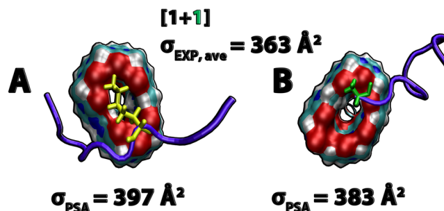
Figure 5. Representative structures of A\beta_{25-35} :CB[7] complexes obtained from simulations. (1 + 1) complexes extracted from the simulation, and their theoretical cross sections. The experimental cross section is an average of the (1 + 1)/2 and (1 + 1)/3 complexes. The CB[7] molecules are represented in filled surface with oxygens in red, carbons in cyan, nitrogens in blue and hydrogens in white. The A\beta_{25-35} peptides are shown in cartoon representation and colored in violet. Lysine (yellow) and N-terminus (green) are shown in licorice representation.
